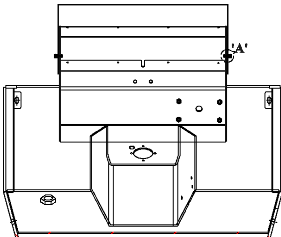
VIEW 'B'
