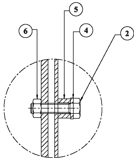
VIEW 'A'
