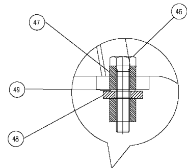
VIEW-L
