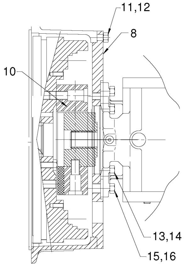
DETAIL X
